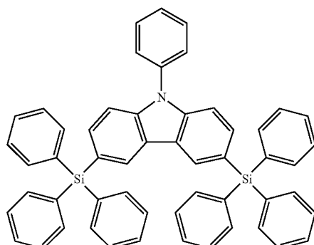
9-(Phenyl)-3,6-bis(triphenylsilyl)carbazole
